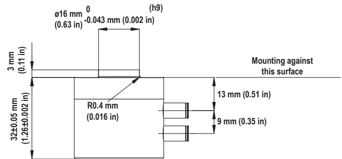
Figure 4. Mounting dimensions of MAP-6
