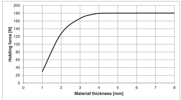
Figure 2. MAP-6 holding force in proportion to material thickness
