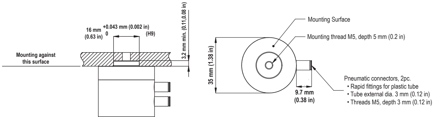
Figure 4. Mounting dimensions of MAP-6
