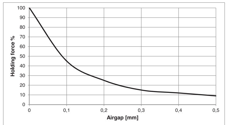
Figure 3. MAP-6 holding force in proportion to airgap
