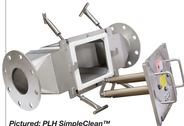
Pictured: PLH SimpleClean™ with custom flanges and mounting design
